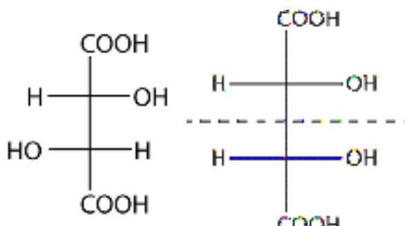
Tartaric acid(I) optically active
